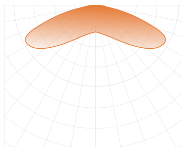
Beam angle: 160°
