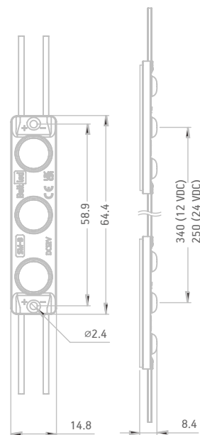
* Dimensions in millimeters
