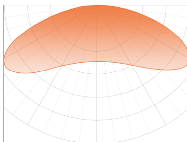
Beam angle: 160°
