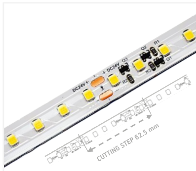
IP 20 | 112 LEDs
