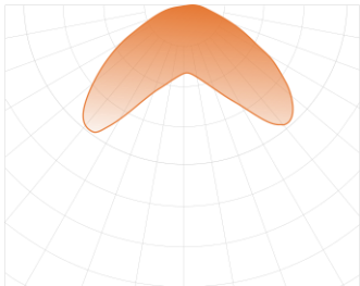
Beam angle: 140°
